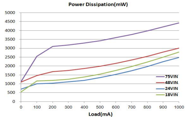
Power Dissipation vs. Load
