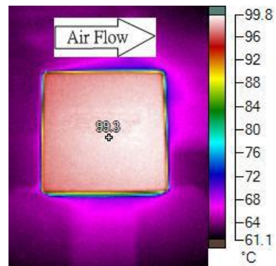
24Vin, 满载, 200LFM, 环温=58°C
