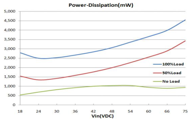
Power Dissipation vs. Input Voltage
