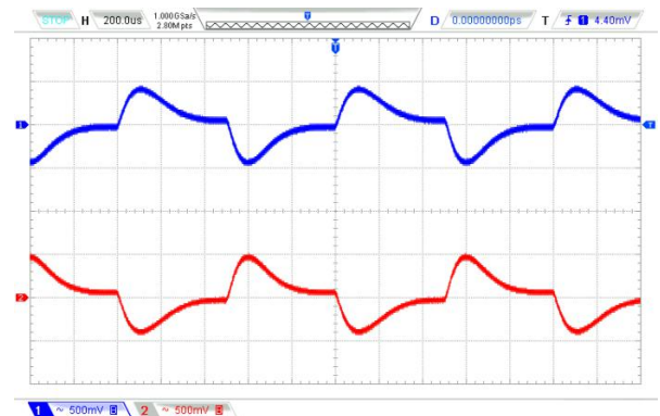
Vin=48VDC @ 50~75%Load
