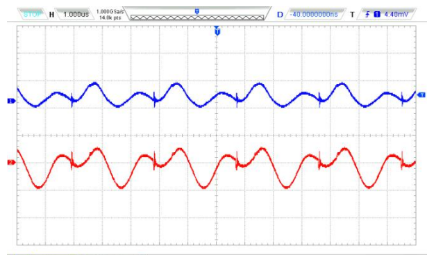
Vin=48VDC @ 100%Load
