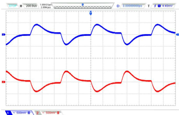
Vin=24VDC @ 50~75%Load
