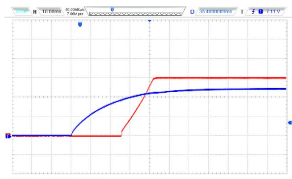
Vin=24VDC @100%Load+3300uF/EC
