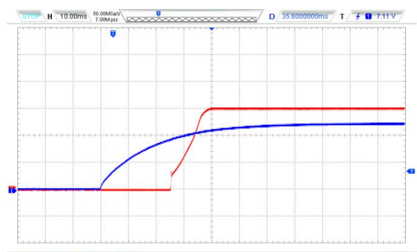
Vin=24VDC @100%Load
