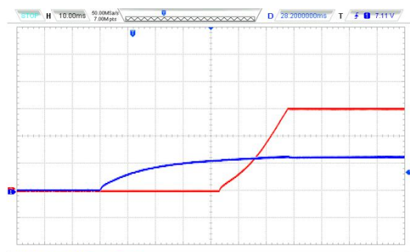
Vin=12VDC @100%Load+3300uF/EC
