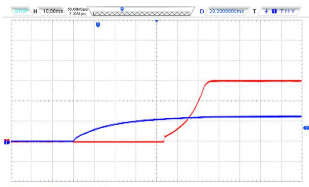
Vin=12VDC @100%Load
