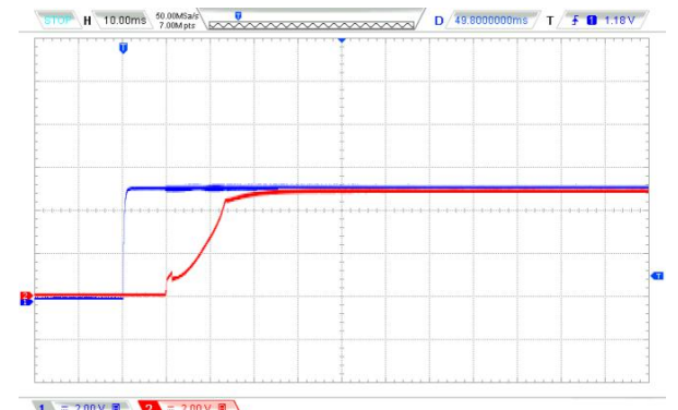
Vin=48VDC @100%Load+1000uF/EC
