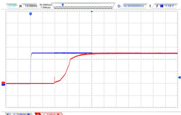
Vin=24VDC @100%Load
