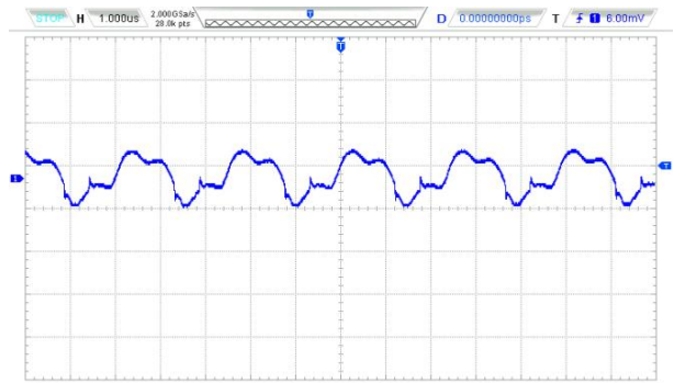
Output Ripple & Noise ,Vin=48VDC @100%Load
