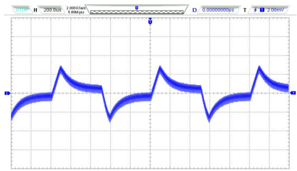
Transient response , 50~75%Load @Vin=48VDC
