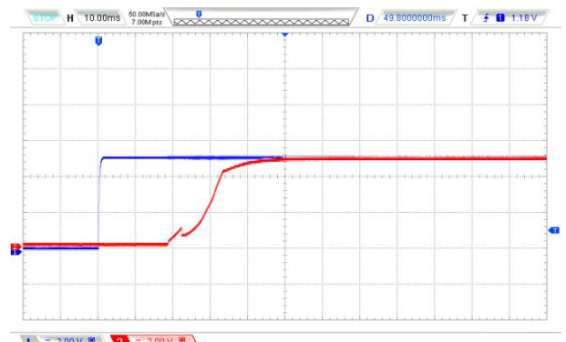
Vin=24VDC @100%Load+1000uF/EC
