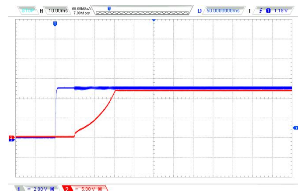
Vin=48VDC @100%Load+4700uF/EC
