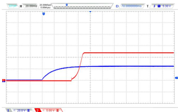
Vin=24VDC @100%Load
