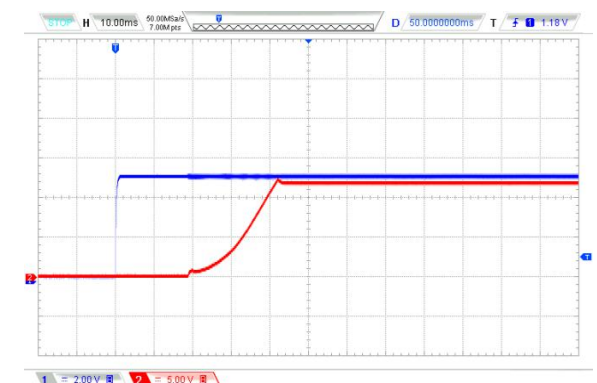
Vin=24VDC @100%Load+4700uF/EC
