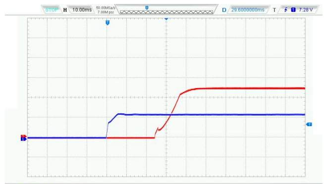
Vin=12VDC @100%Load+1000uF/EC
