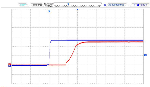
Vin=12VDC @100%Load
