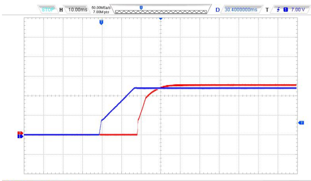
Vin=24VDC @100%Load
