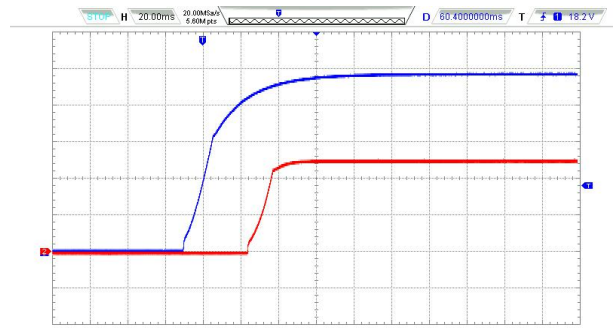
Vin=48VDC @100%Load +10000uF/EC
