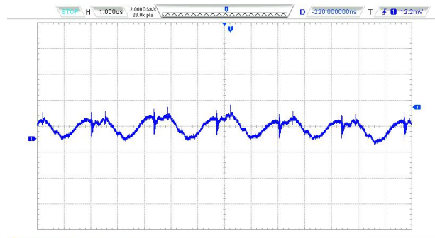
Output Ripple & Noise @ Vin=48VDC, 100% Load
