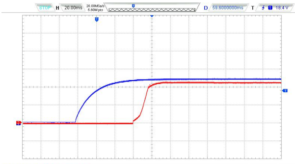
Vin=24VDC @100%Load
