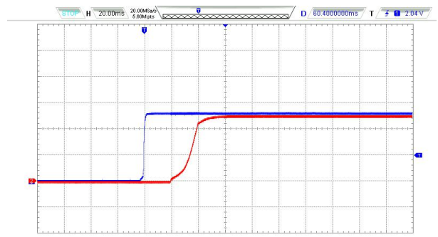
Vin=24VDC @100%Load +10000uF/EC
