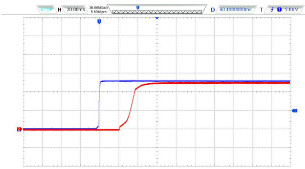
Vin=24VDC @100%Load
