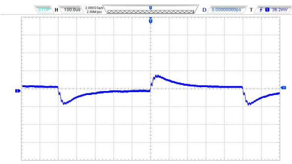
Transient response @ 50~75% Load, Vin=24VDC
