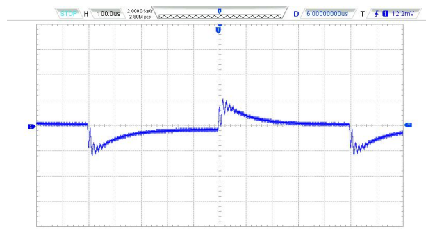
Transient response @ 50~75% Load, Vin=48VDC
