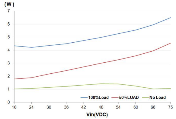
Power Dissipation vs. Input Voltage
