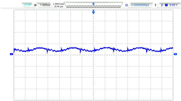
Output Ripple & Noise ,Vin=24VDC @100%Load
