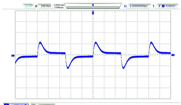
Transient response , 50~75%Load @Vin=48VDC
