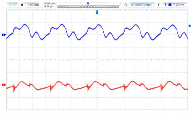
Vin=12VDC @100%Load
