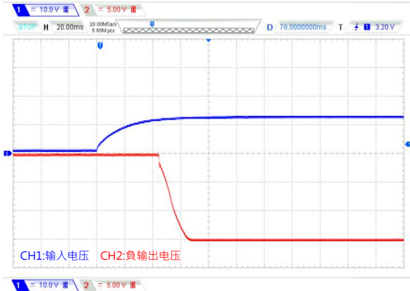
Vin=12VDC @100%Load
