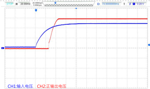
Vin=12VDC @100%Load
