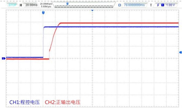
Vin=12VDC @100%Load
