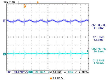
输入电流纹波/输出电压纹波噪声 ( V_{IN} : 24V, Load: 100%, L_{in} =10 \mu H / C_{in} =470 \mu F)
