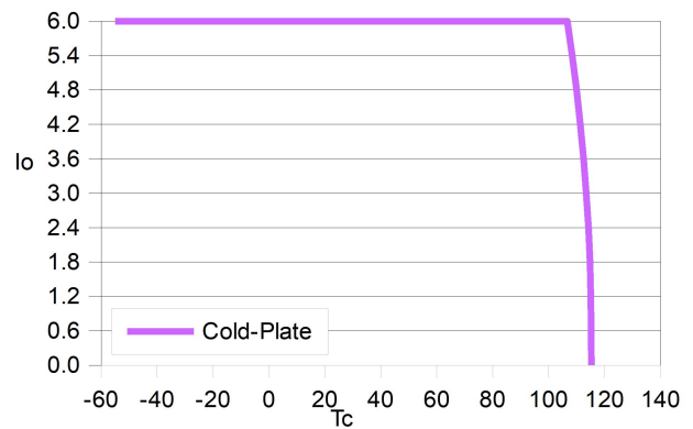
降额曲线(外加液冷板) ( T_c = 120^{\circ}\text{C}/\text{OTP} )
