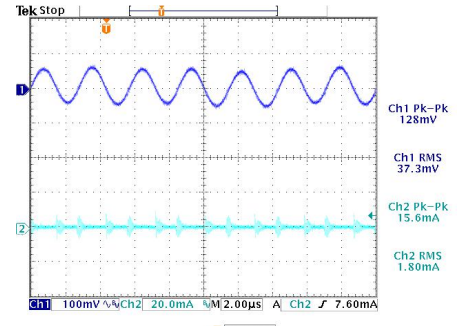
输入电流纹波/输出电压纹波噪声 ( V_{IN} : 24V, Load: 100%, L_{in} =10 \mu H / C_{in} =470 \mu F)
