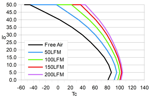
降额曲线(单体无外加散热片) ( T_c = 120^{\circ}\text{C}/\text{OTP} )
