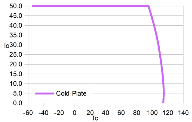
降额曲线(外加液冷板) ( T_c = 120^{\circ}\text{C}/\text{OTP} )
