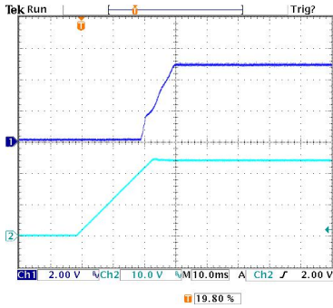
启动波形 (Power ON / V_{IN} : 24V, Load: 100%)
